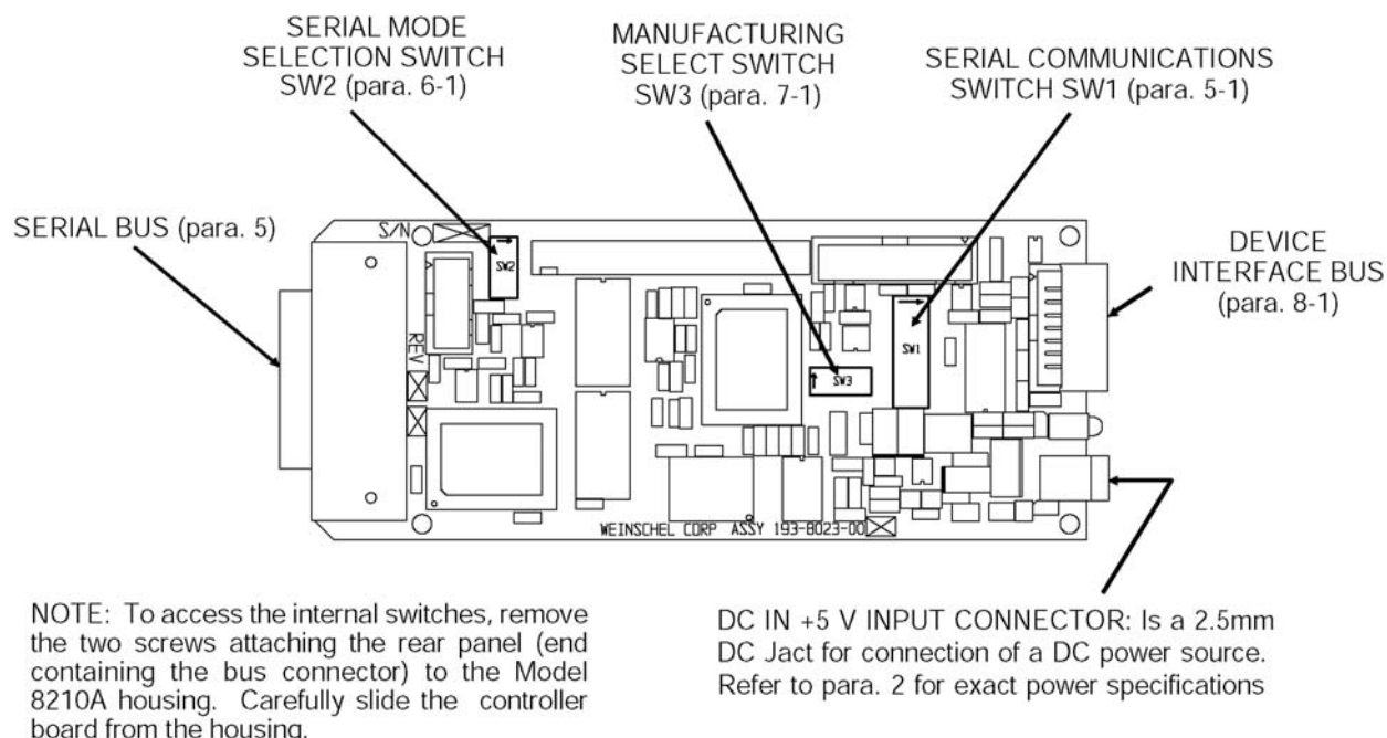
Figure 4. Model 8210A-2-5 Internal Switch Locations
